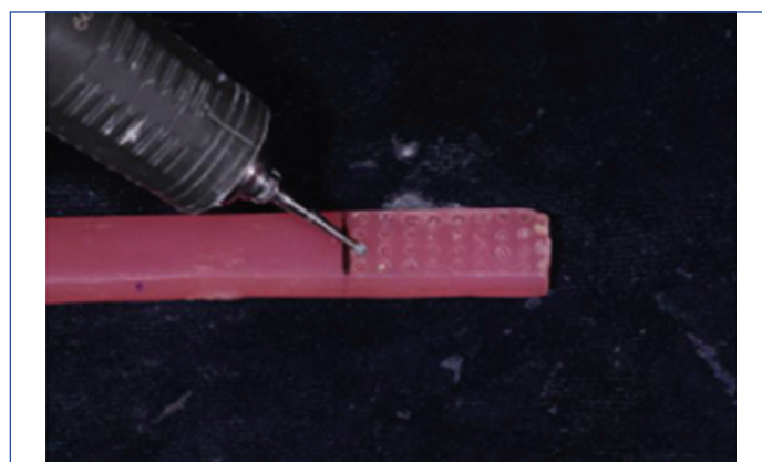
[Table/Fig-3]: Retentive holes measuring 1.5 mm in diameter and 0.5 mm in depth.
